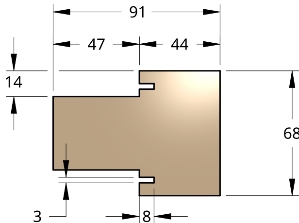
MULLION
